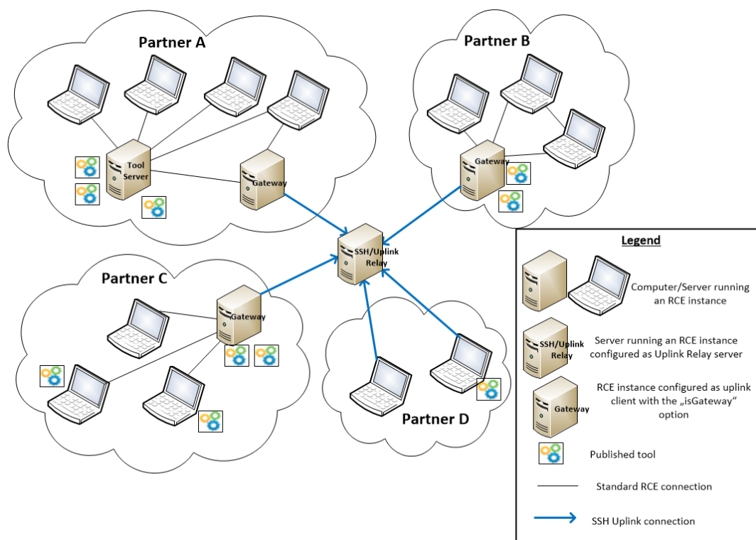
Figure 3.9. Example RCE network
